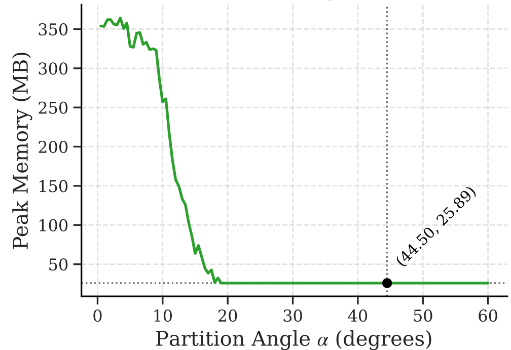
Peak Memory vs. \alpha
