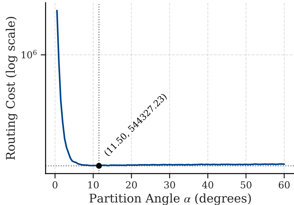
Cost vs. \alpha
