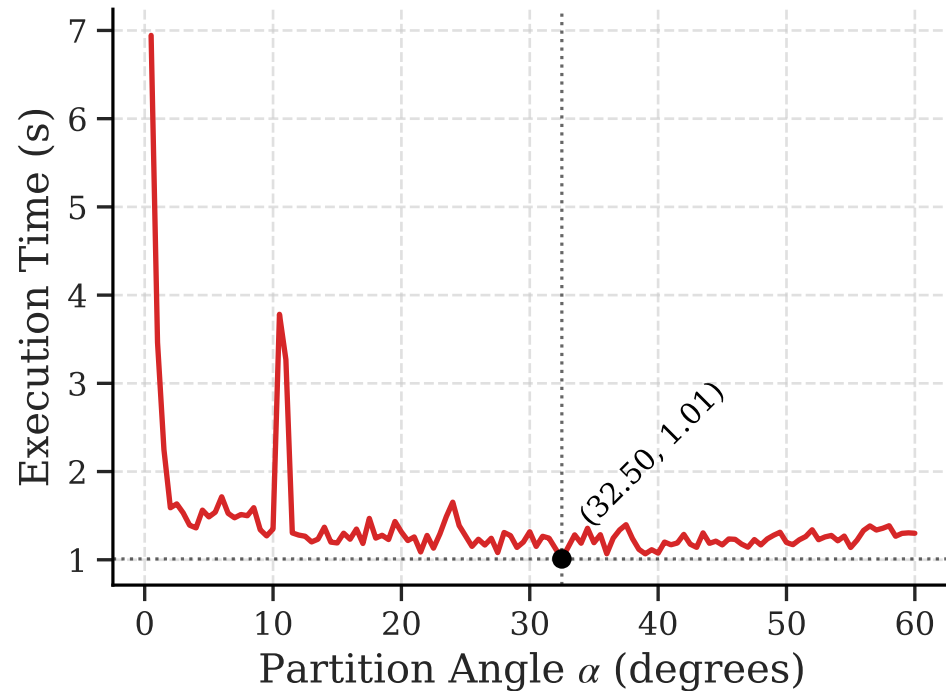
Execution Time vs. \alpha
