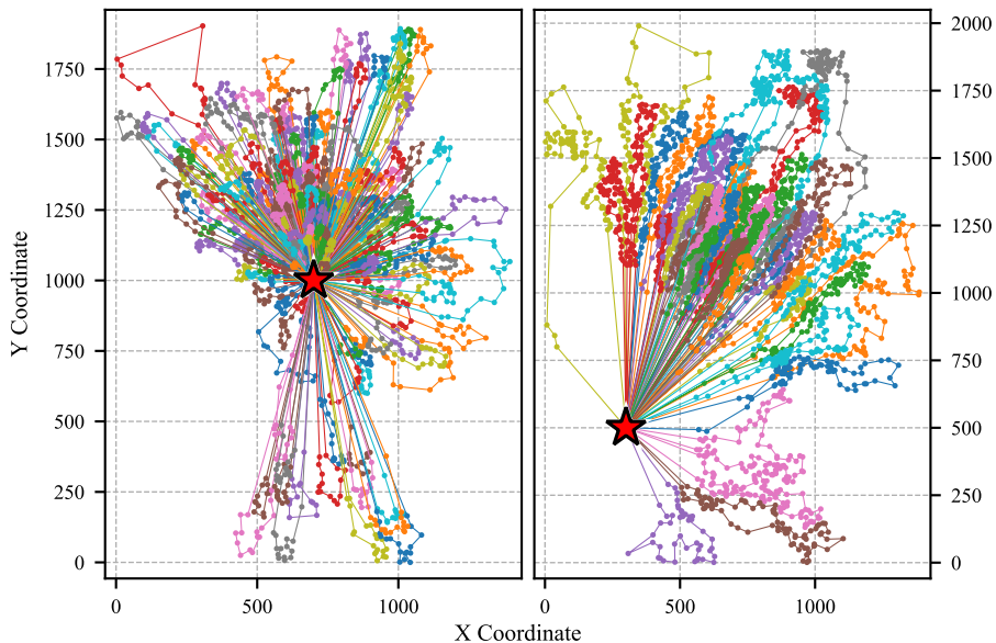
(a) Leuven1 — Cost: 192848
