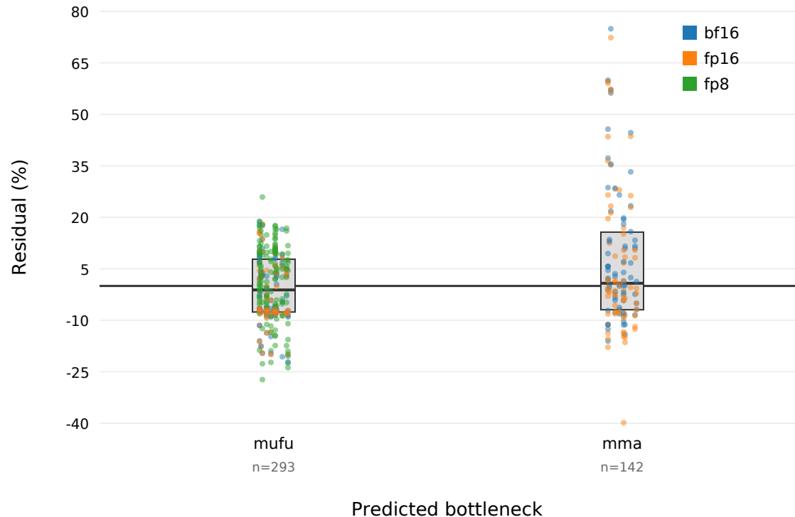
Figure 2: Residual distribution by predicted bottleneck
