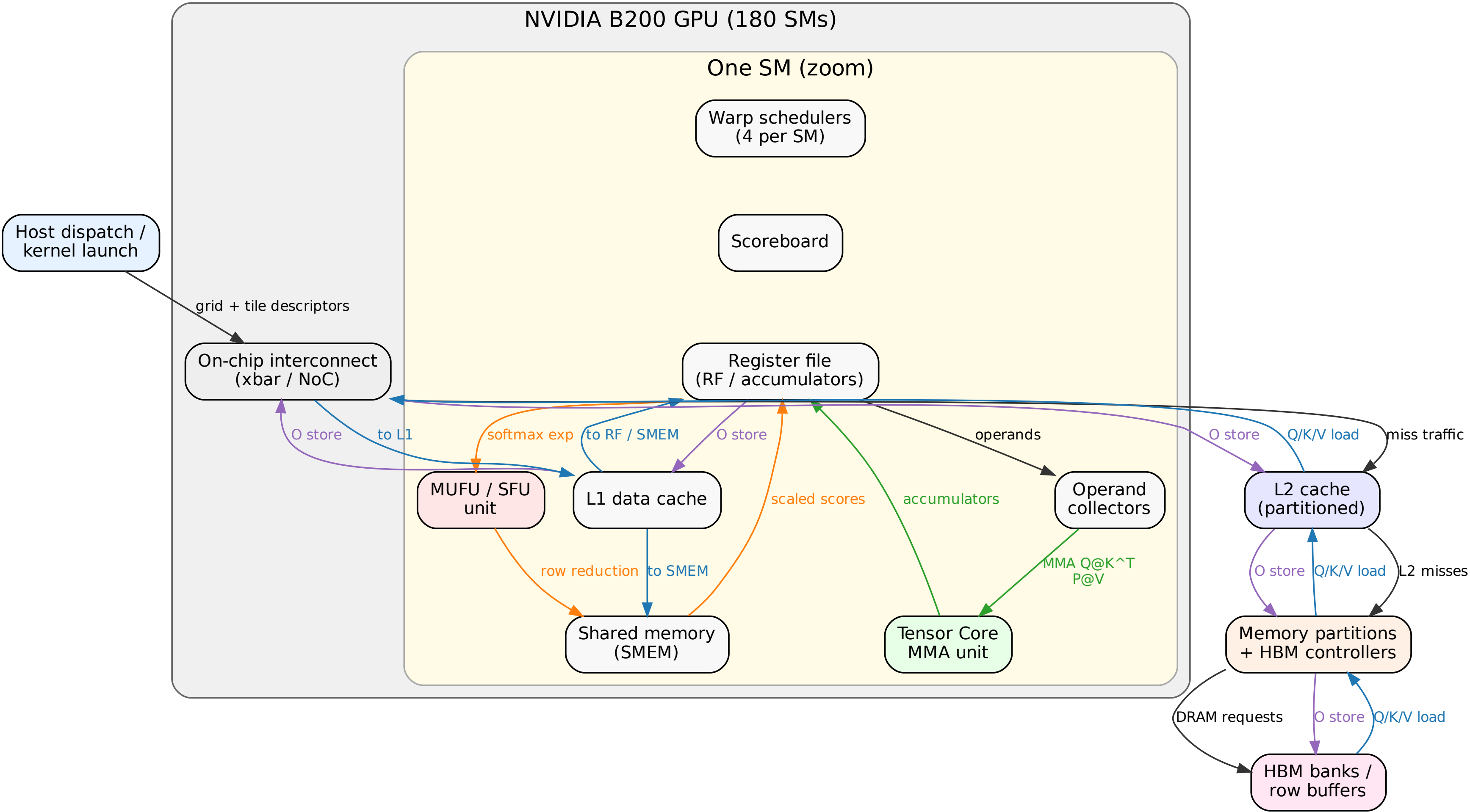
Figure 4: GPU hardware component execution system for FA4 on B200
