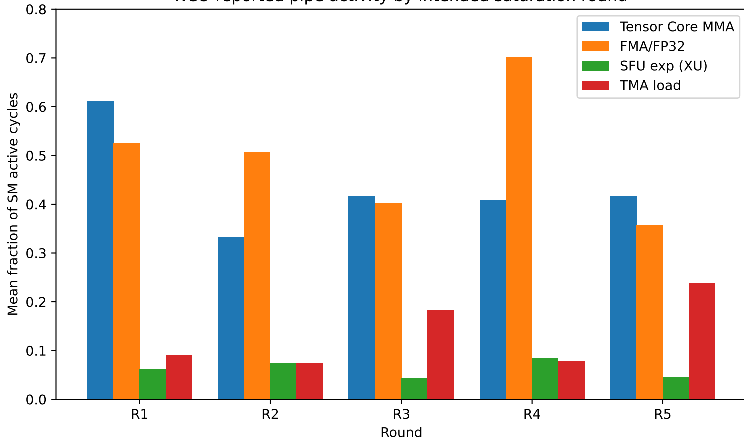
NCU-reported pipe activity by intended saturation round
