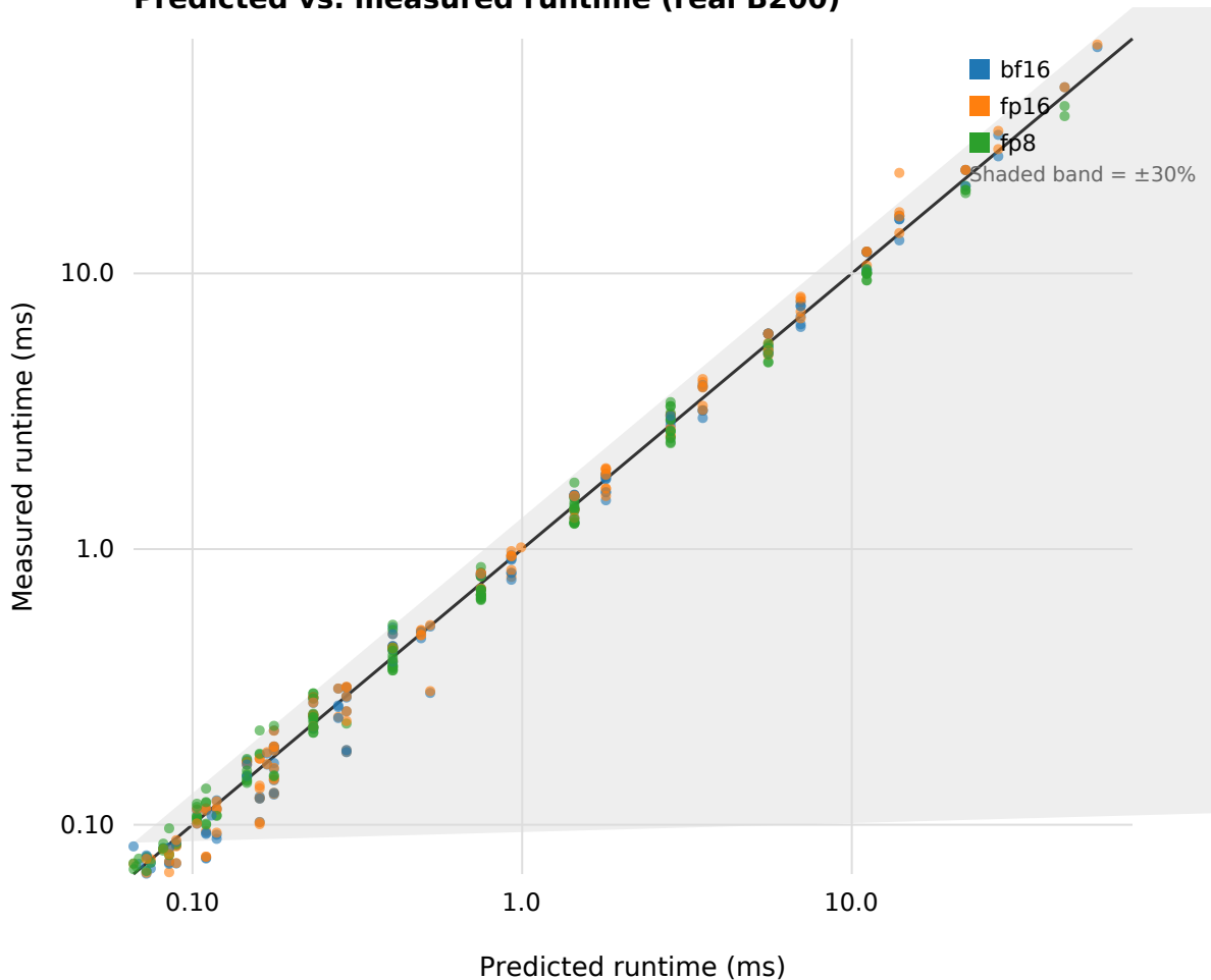
Predicted vs. measured runtime (real B200)
