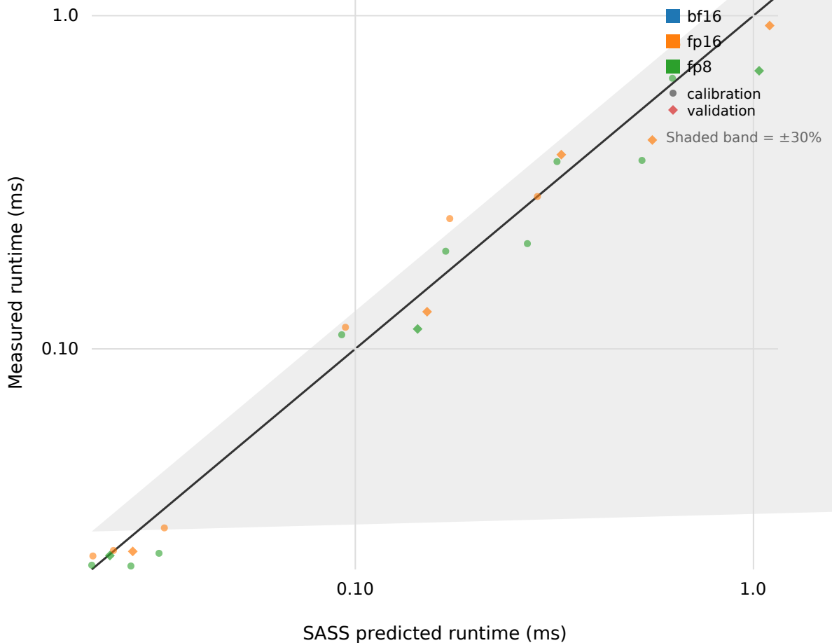
Predicted vs. measured runtime (SASS critical-path model)
