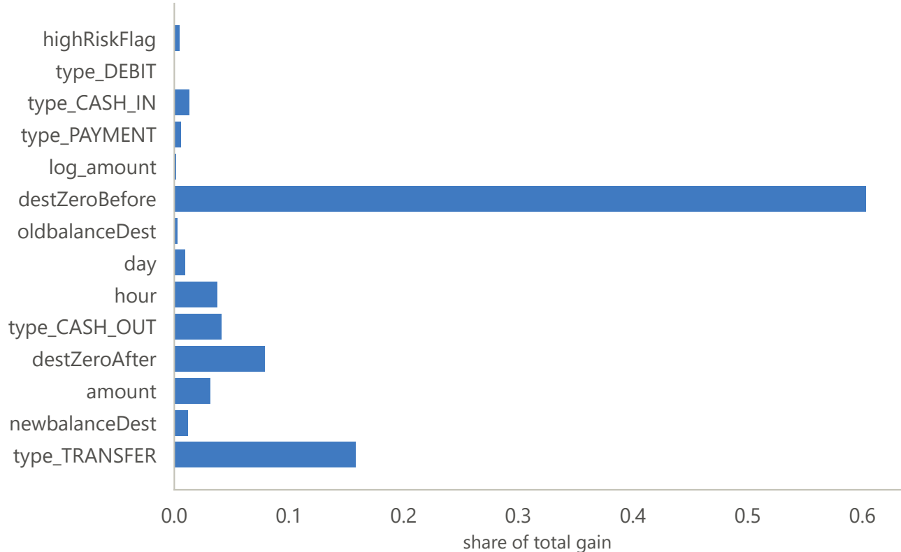
Gain — where the trees split
