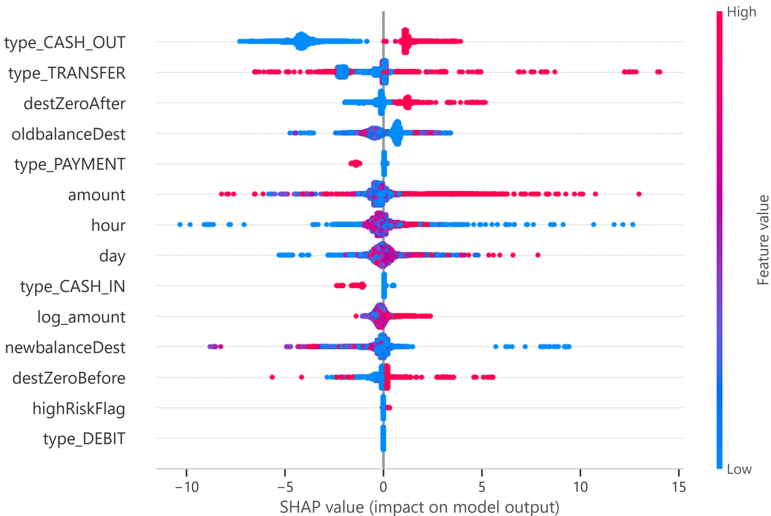
SHAP — contribution to the fraud score, per transaction
