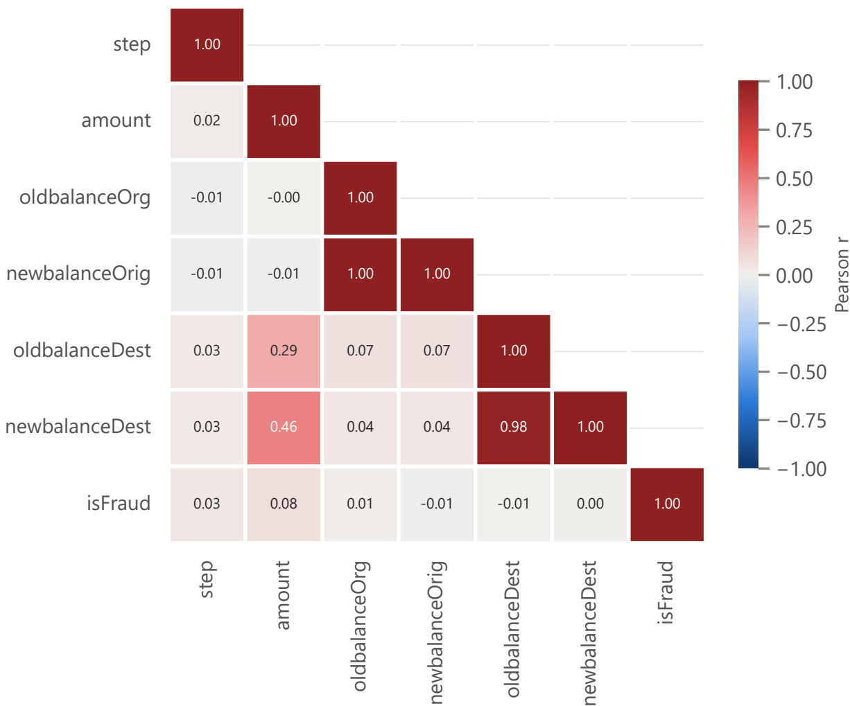
Raw feature correlations
