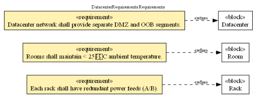
Figure 1: Requirement diagram
