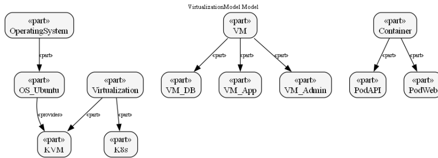
Figure 5: Block definition diagram
