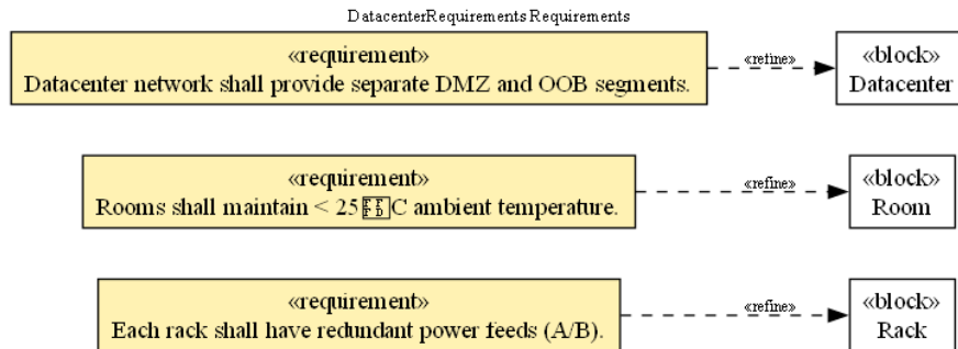
Figure 3: Requirement diagram
