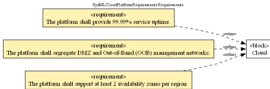
Figure 10: Requirement diagram
