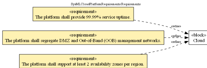
Figure 3: Requirement diagram
