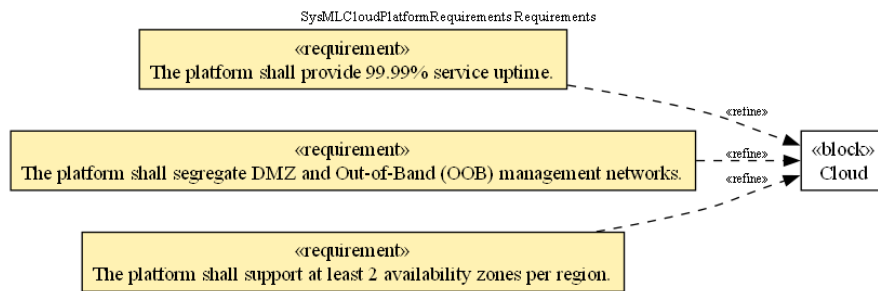
Figure 19: Requirement diagram
