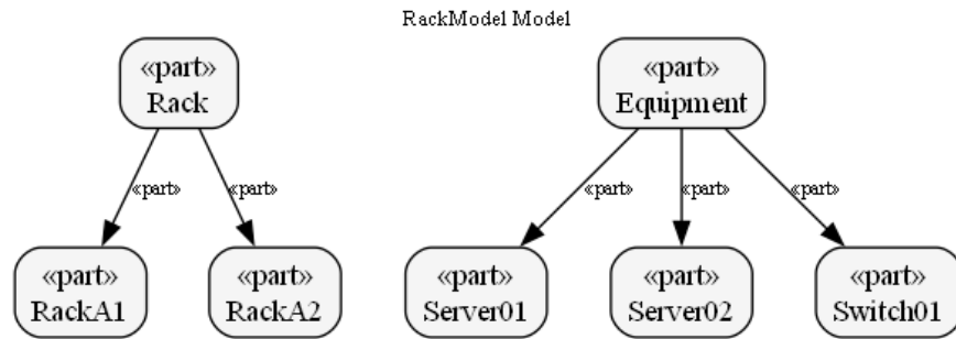
Figure 18: Block definition diagram
