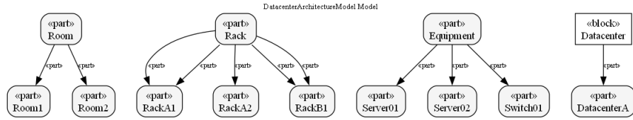
Figure 2: Block definition diagram
