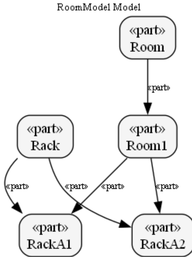
Figure 20: Block definition diagram
