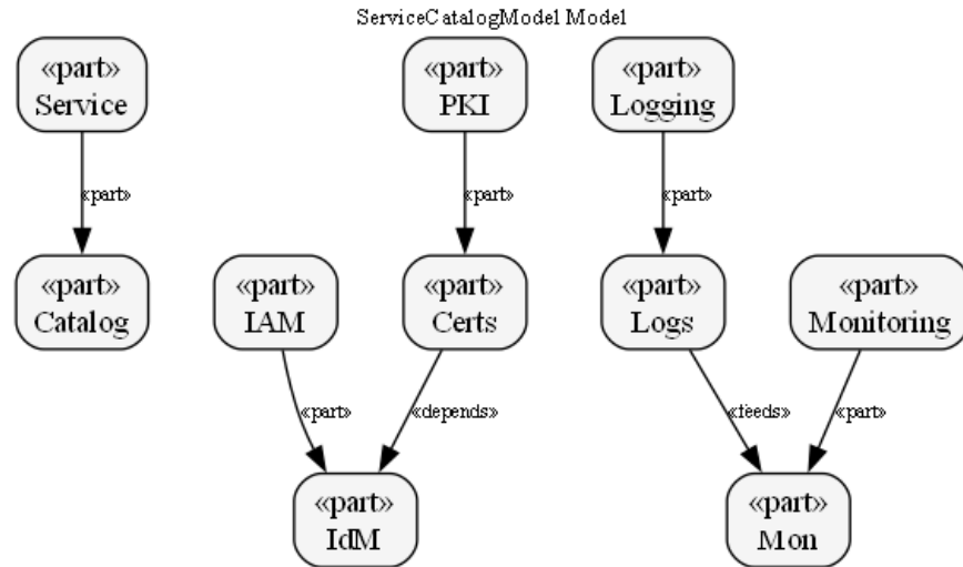
Figure 21: Block definition diagram
