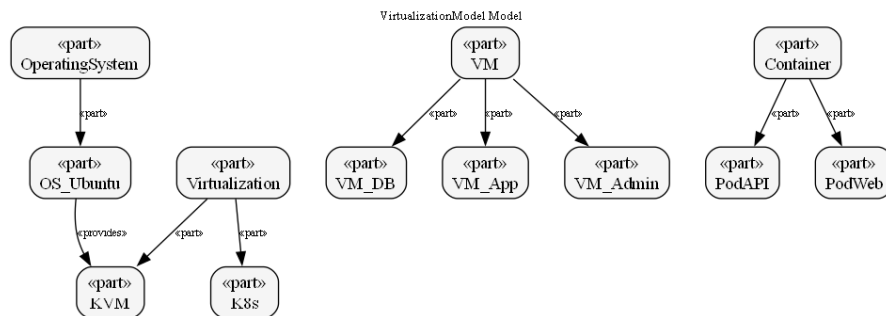
Figure 28: Block definition diagram
