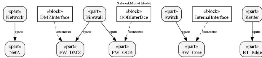
Figure 11: Block definition diagram
