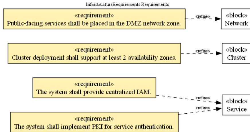
Figure 8: Requirement diagram
