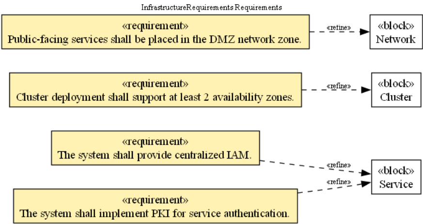
Figure 1: Requirement diagram
