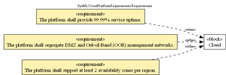
Figure 1: Requirement diagram
