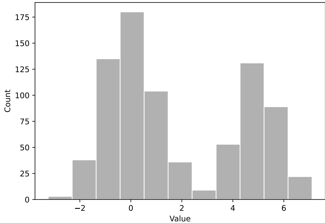
Sturges rule: 11 bins
