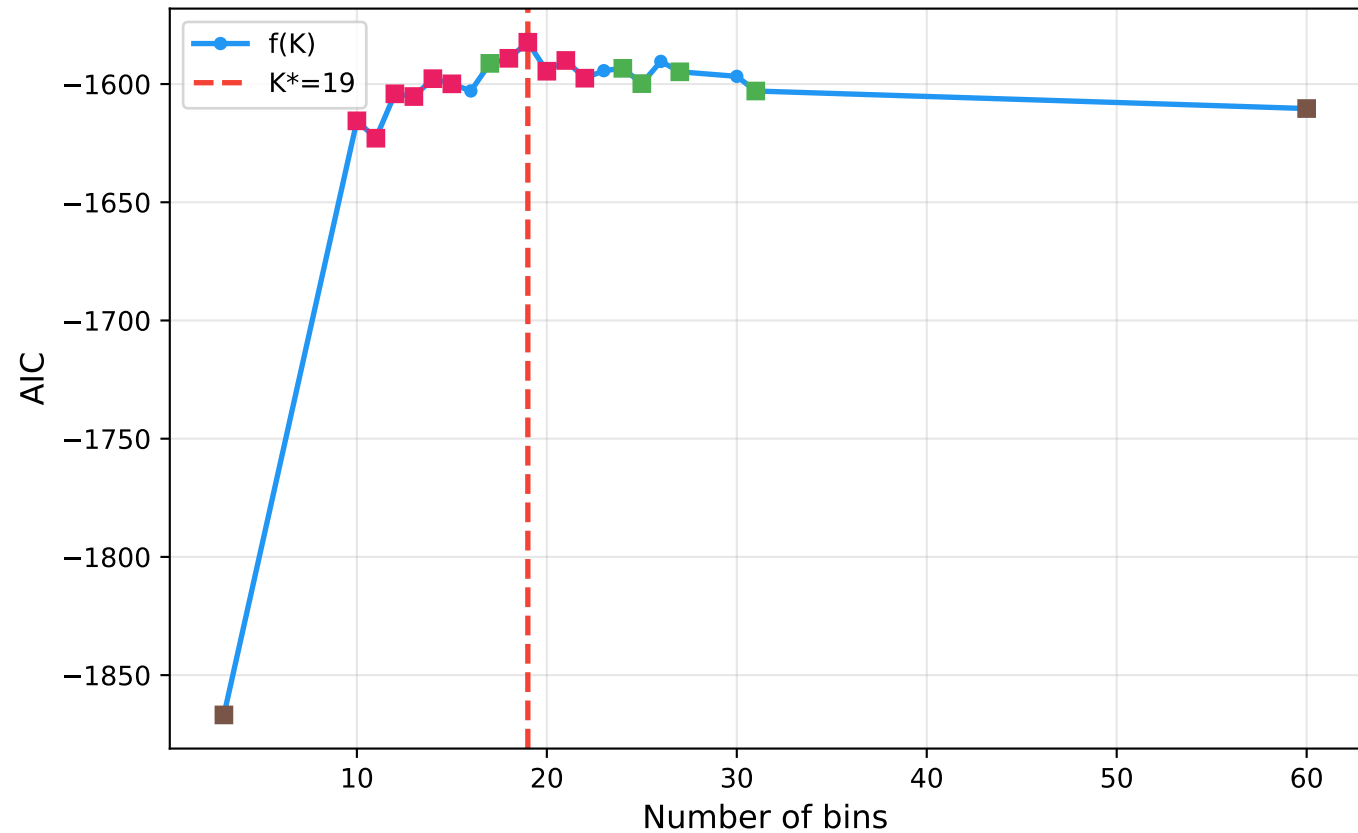
NumPy: Optimal Histogram Bins (AIC, binary search)
