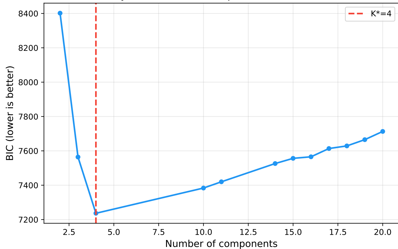
SciPy/sklearn: GMM Component Selection (BIC)
