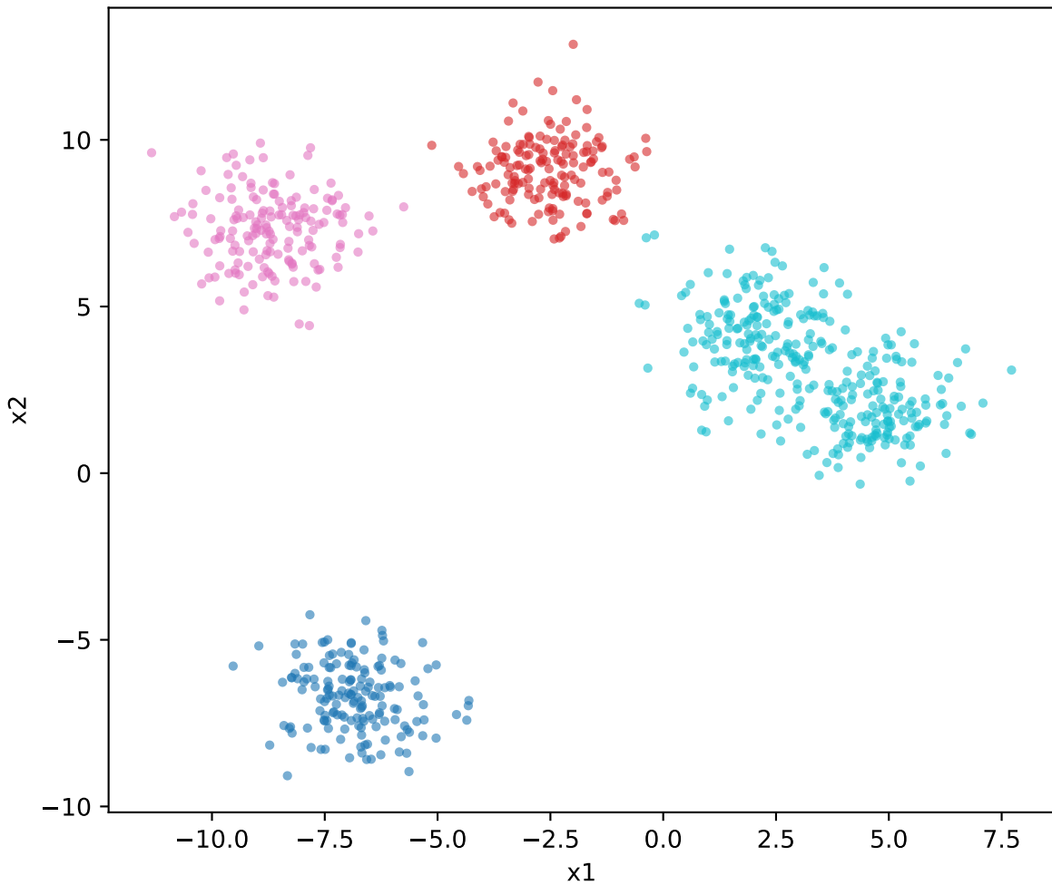
GMM with 4 components
