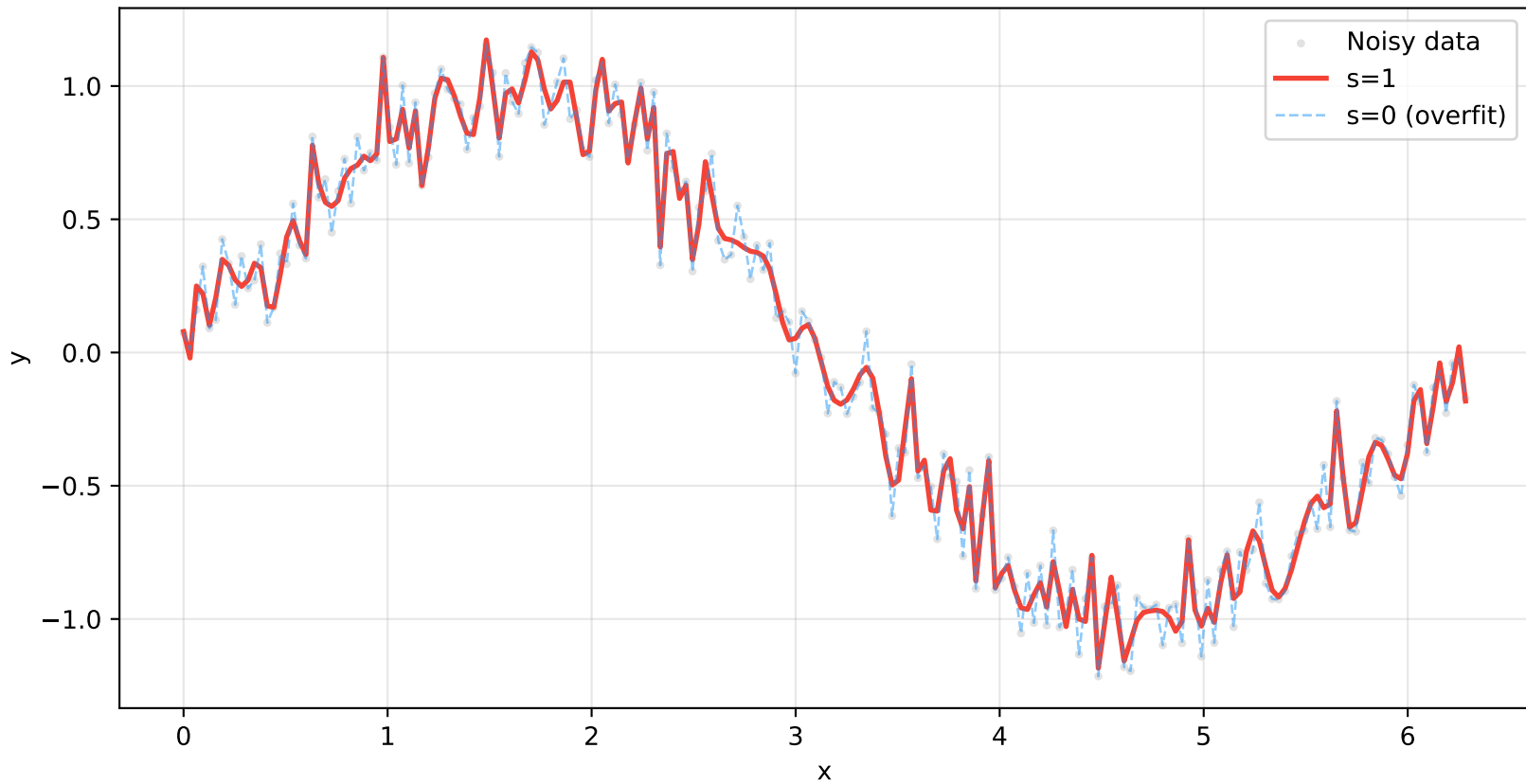
SciPy: Smoothing Spline with ATCND-selected parameter
