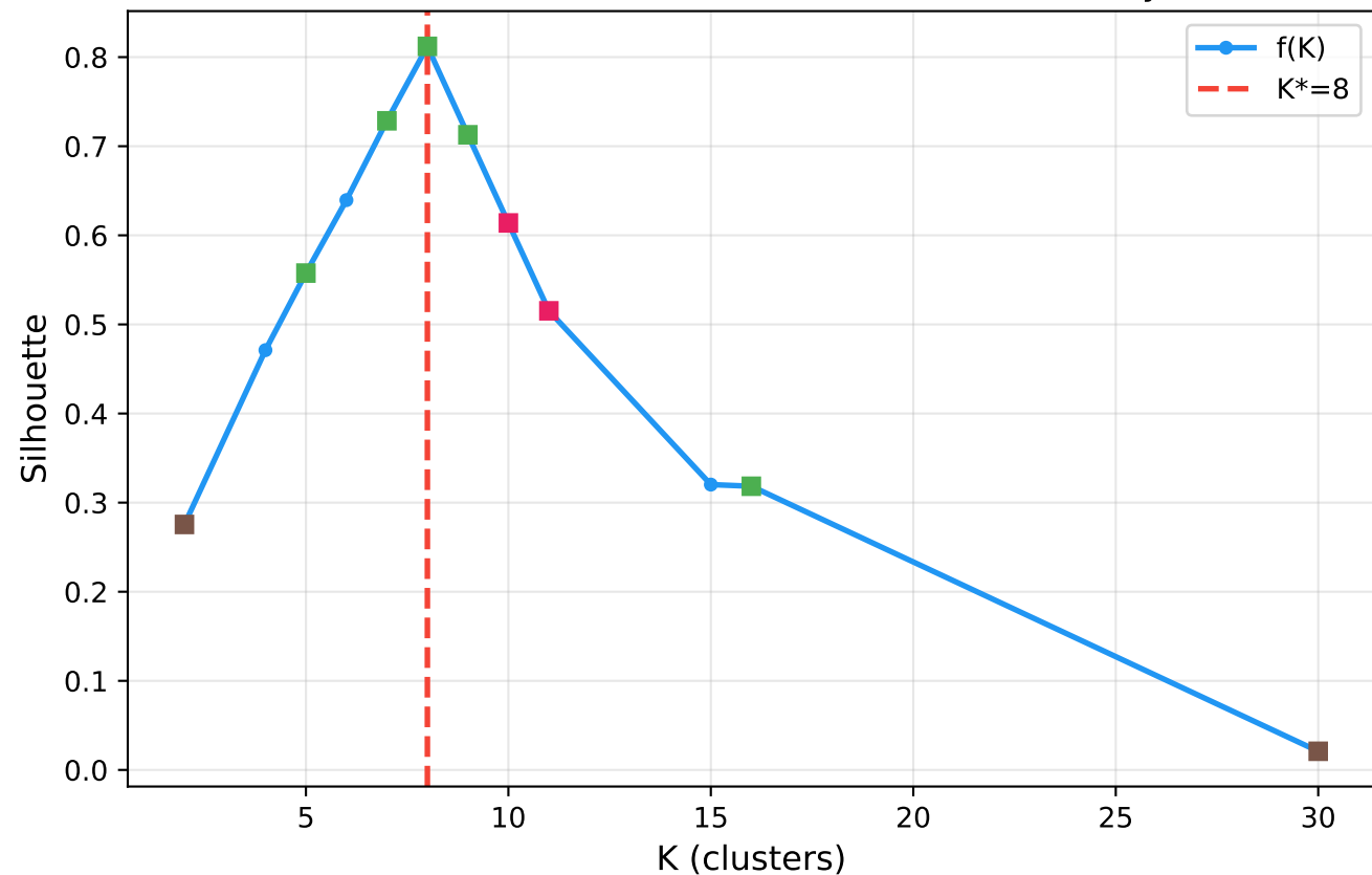
sklearn: K-Means Cluster Selection (silhouette, binary search)
