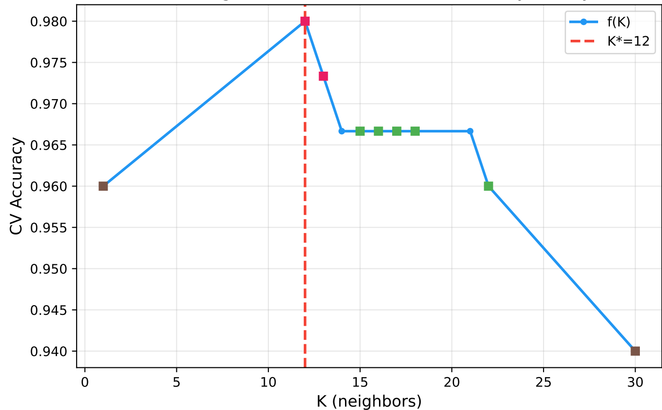
sklearn: KNN Neighbor Selection (5-fold CV accuracy, binary search)
