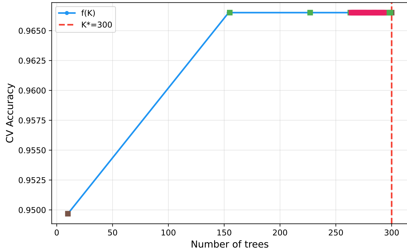
sklearn: Random Forest Tree Count (5-fold CV, binary search)
