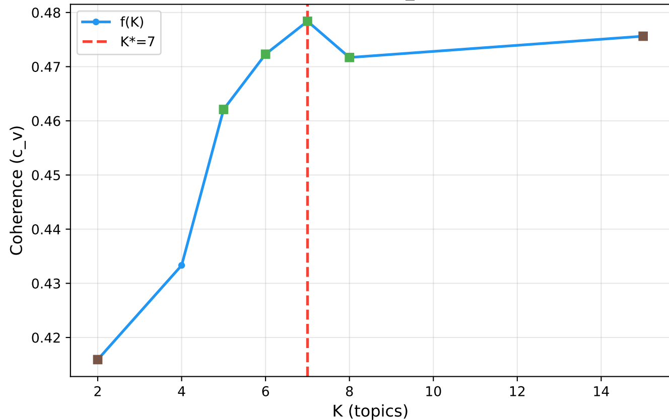
Gensim+sklearn: NMF Topic Count ( c_v coherence, binary search)
