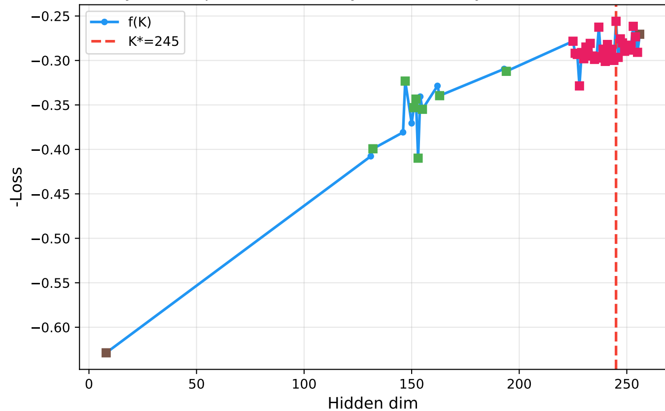
PyTorch: Optimal Hidden Layer Size (binary search, -CE loss)
