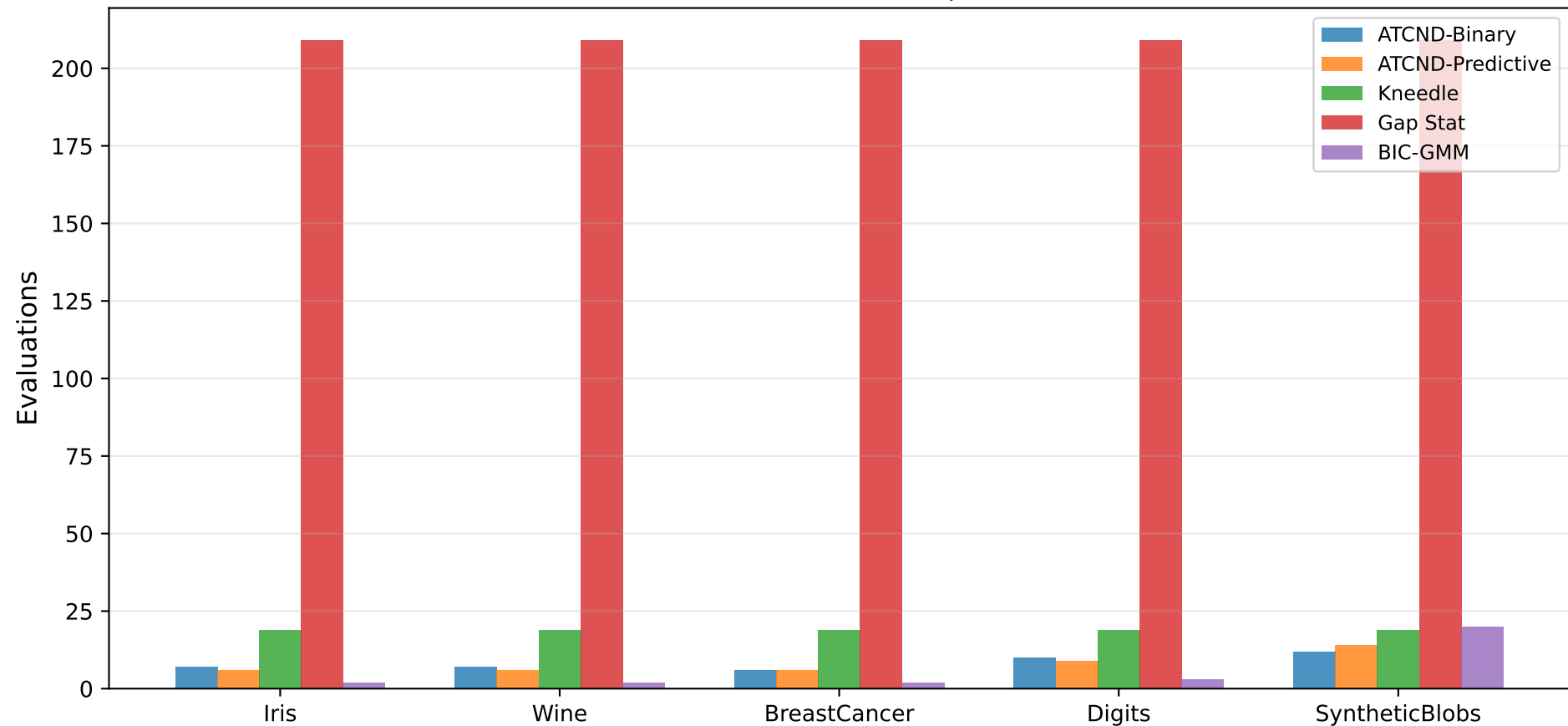
Evaluation Count Comparison
