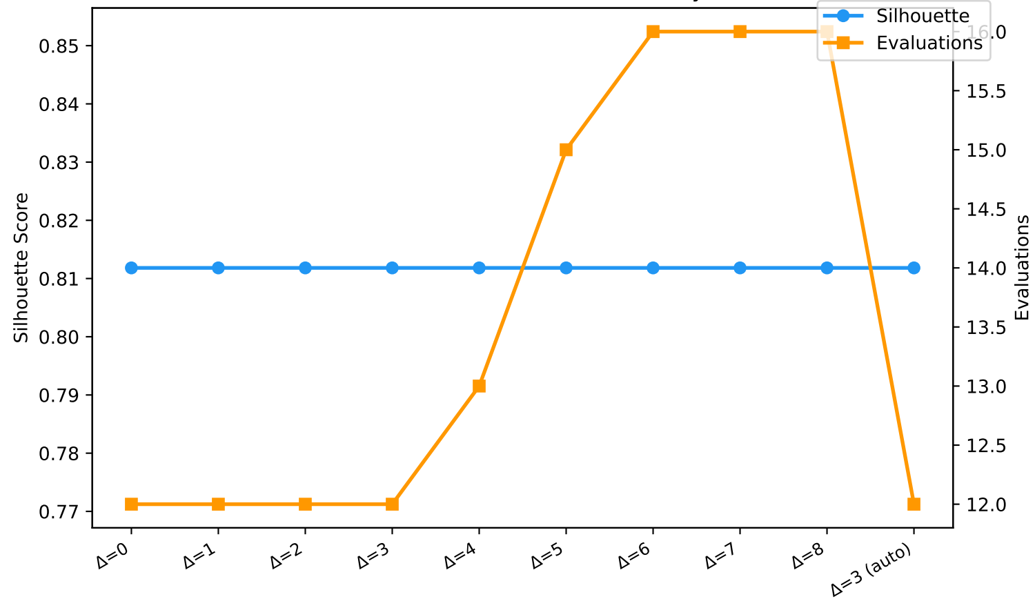
Ablation: \Delta Parameter Sensitivity
