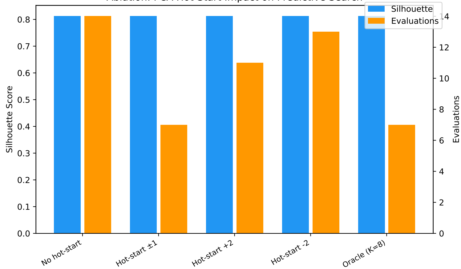
Ablation: PCA Hot-Start Impact on Predictive Search
