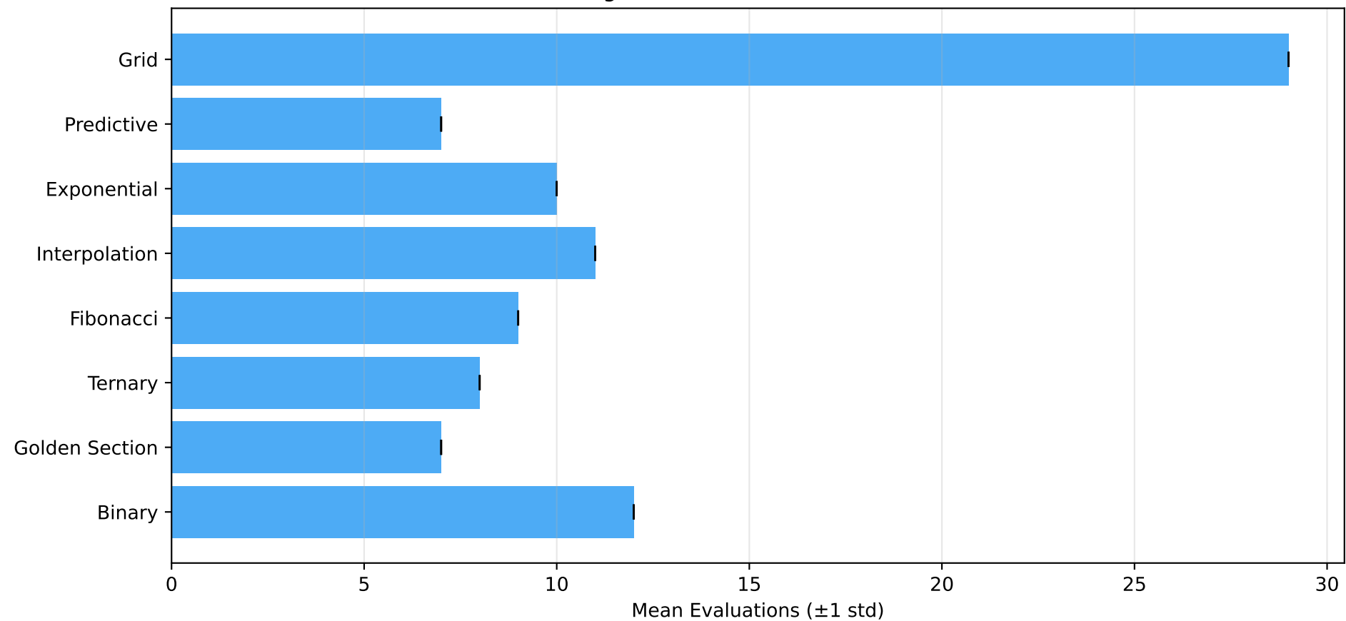
Statistical Significance: Evaluation Counts (10 runs)
