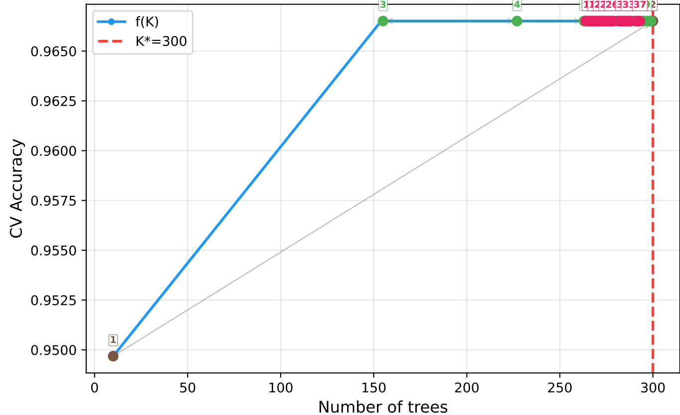
sklearn: Random Forest Tree Count on Wine (5-fold CV)
