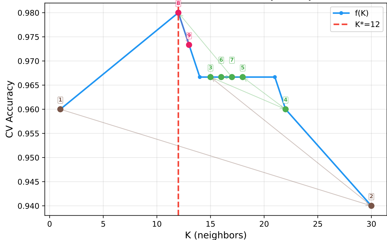
sklearn: KNN on Iris (5-fold CV accuracy, binary search)
