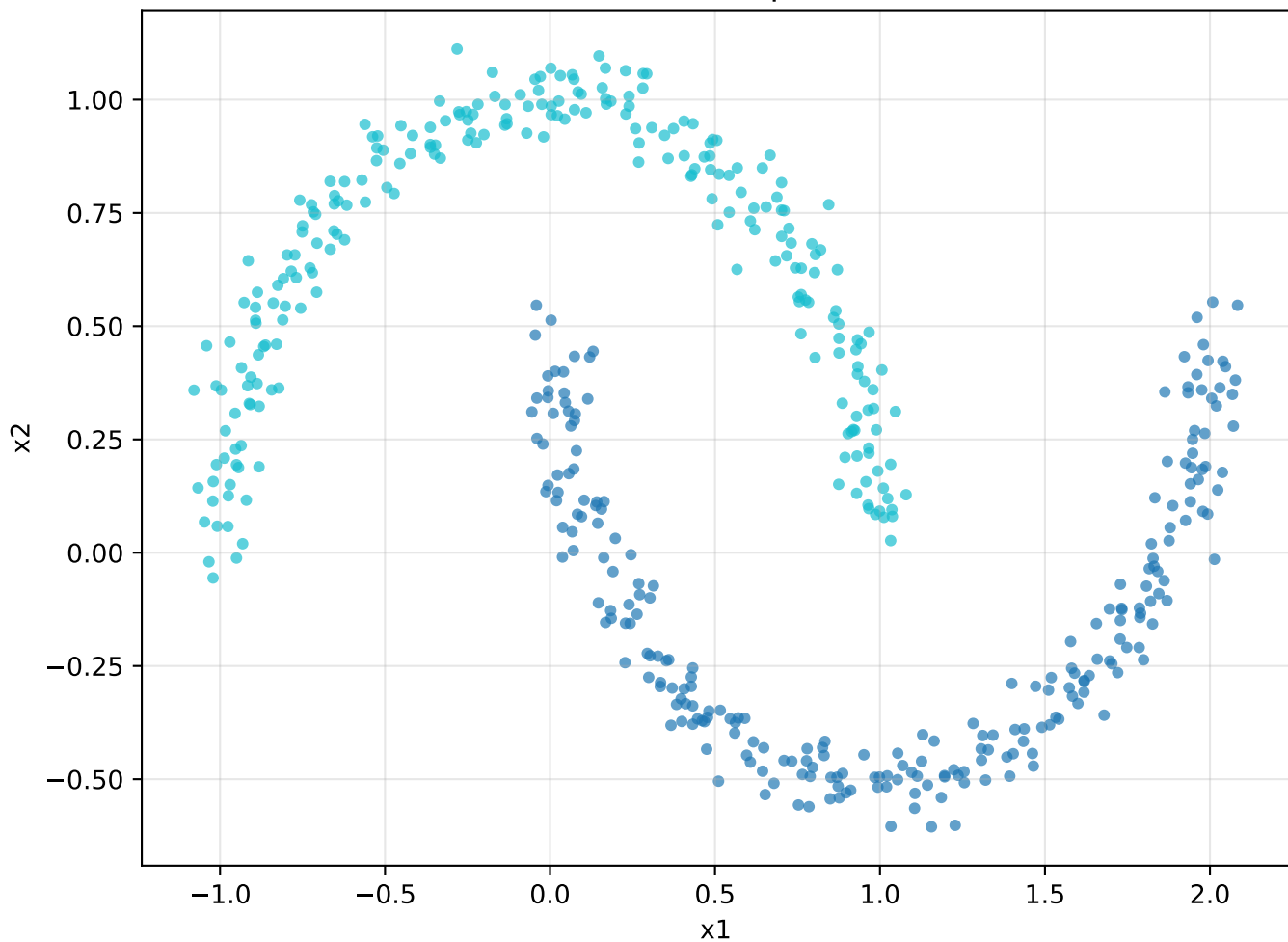
Two-Moons: DBSCAN eps=0.3 (ATCND)
