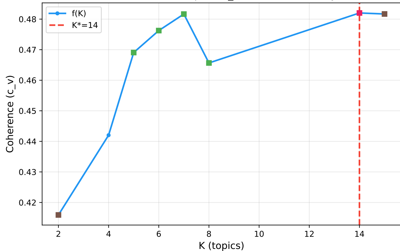
Gensim+sklearn: NMF Topics (c_v coherence, binary search)
