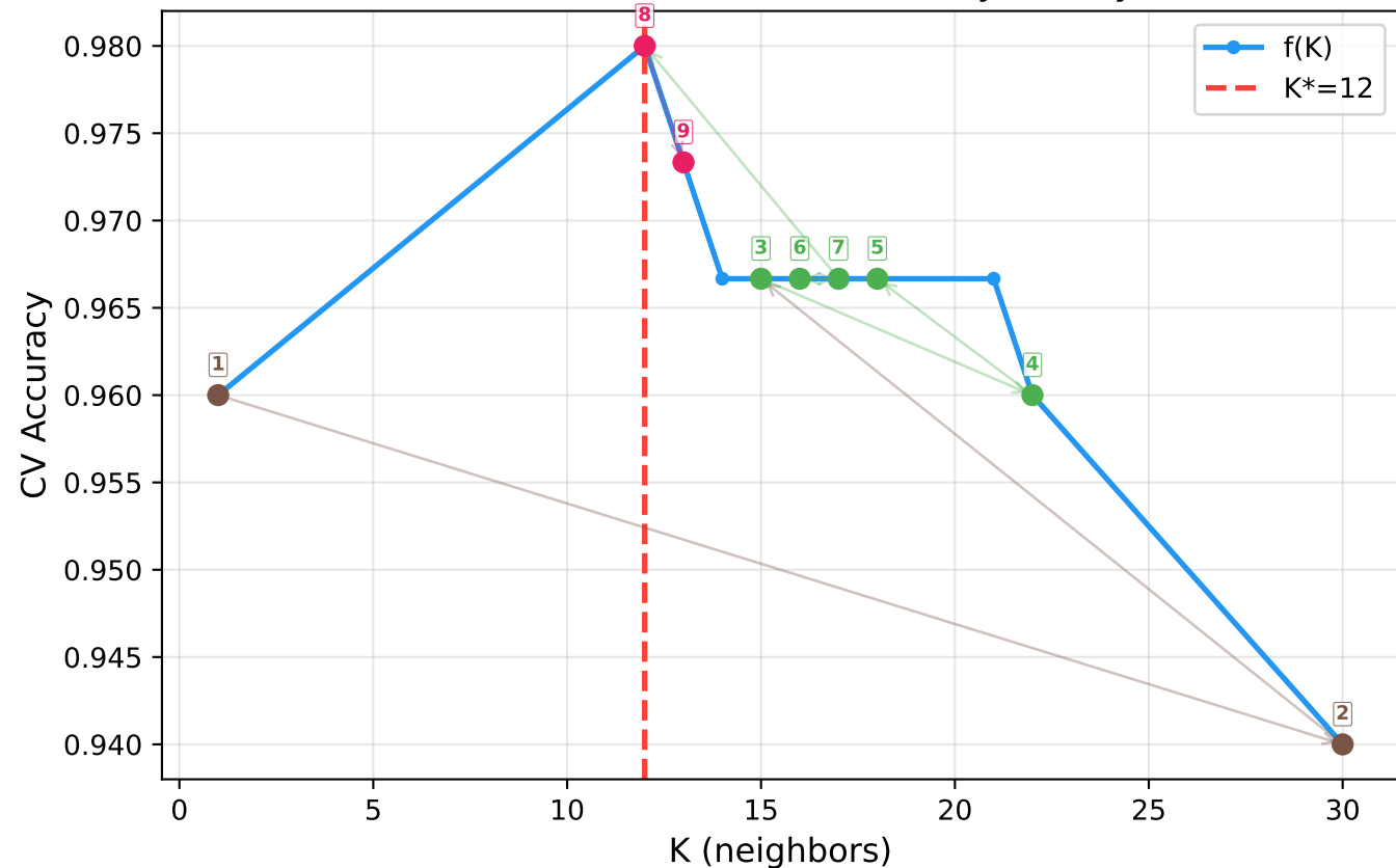
sklearn: KNN on Iris (5-fold CV accuracy, binary search)
