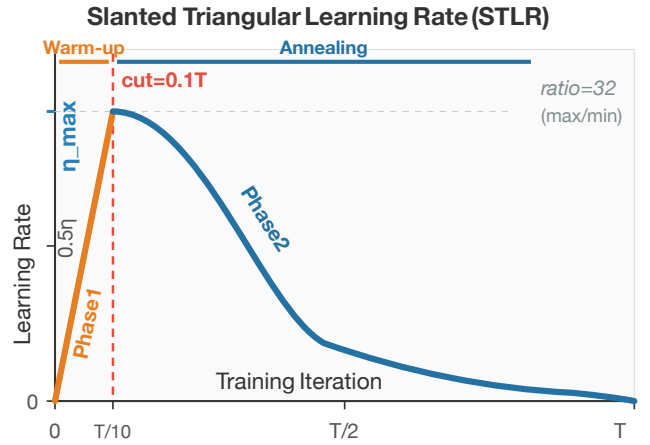
Figure 4: STLR combines rapid warmup (first 10%) with gradual decay (remaining 90%), creating the characteristic slanted triangular shape.
