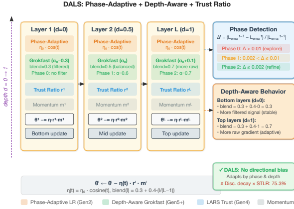
Figure 5: The DALS pipeline—loss-based phase detection drives gradient smoothing intensity, depth-aware blending controls raw vs. filtered gradient ratio, and trust ratio normalizes per-parameter updates.
