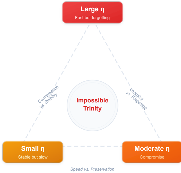
Figure 1: The impossible trinity—no single global \eta can simultaneously achieve fast convergence, knowledge preservation, and optimal performance across all layers.
