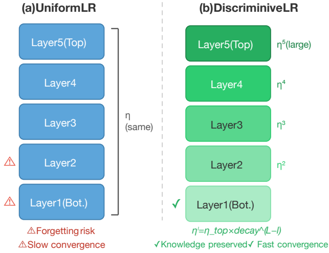
Figure 3: Feature hierarchy—lower layers capture general features requiring smaller updates, higher layers encode task-specific concepts requiring larger updates.
