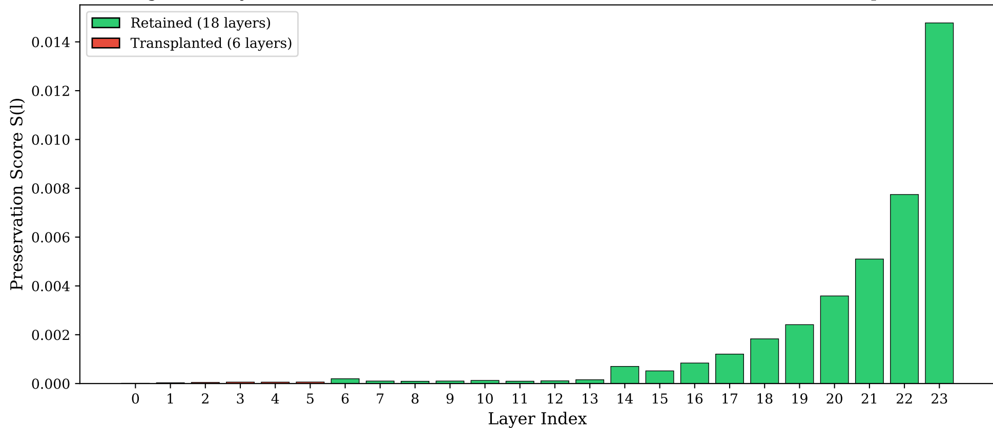
Figure 2: Layer Preservation Score for Profile P1 (Green = Retained, Red = Transplanted)
