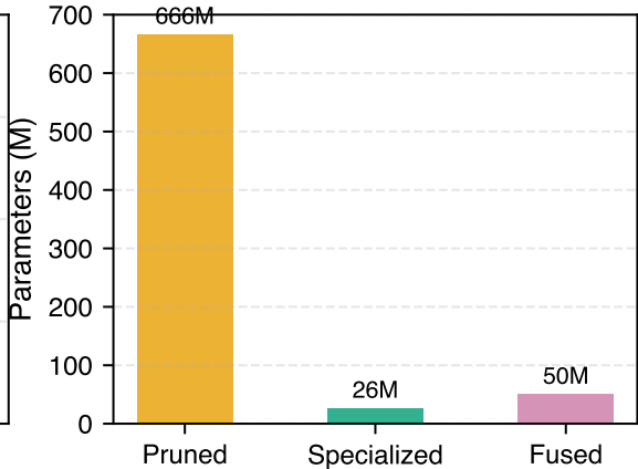
Model Size
