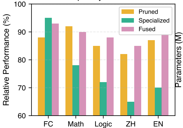
Capability Retention
