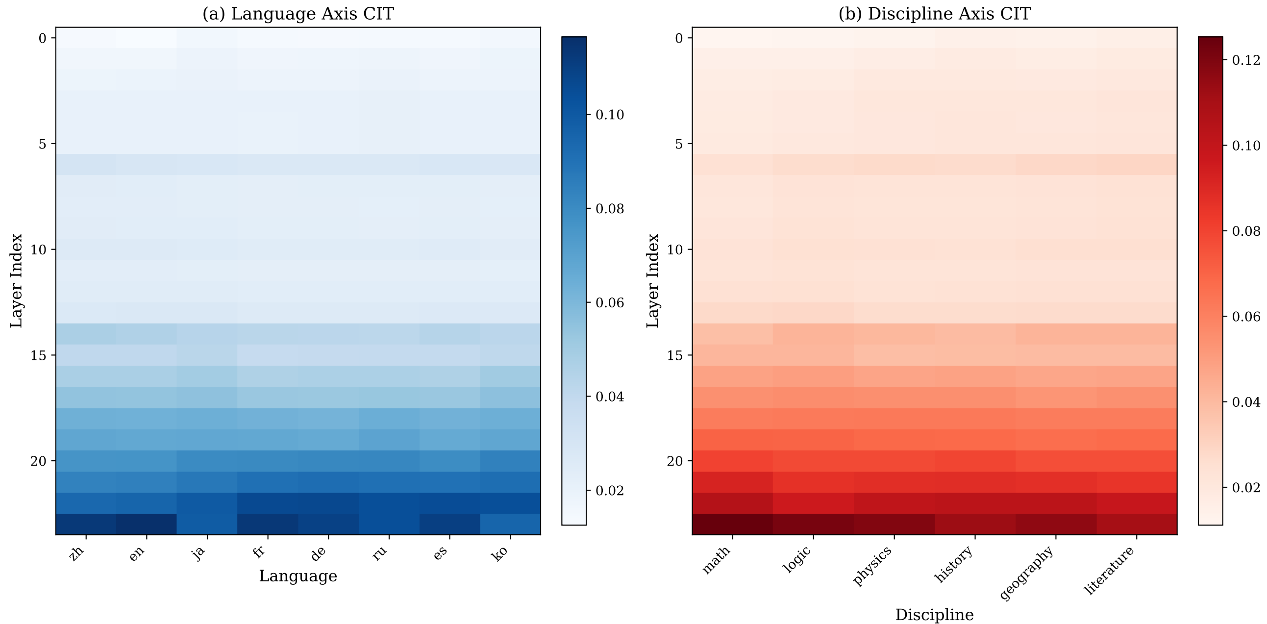
Figure 4: Capability Cliff — Layer Importance Rises Sharply at Layers 14-23
