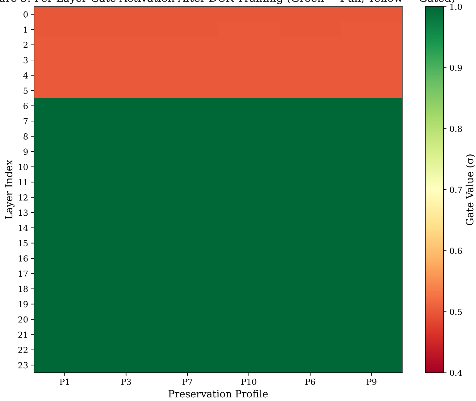
Figure 5: Per-Layer Gate Activation After DCR Training (Green = Full, Yellow = Gated)
