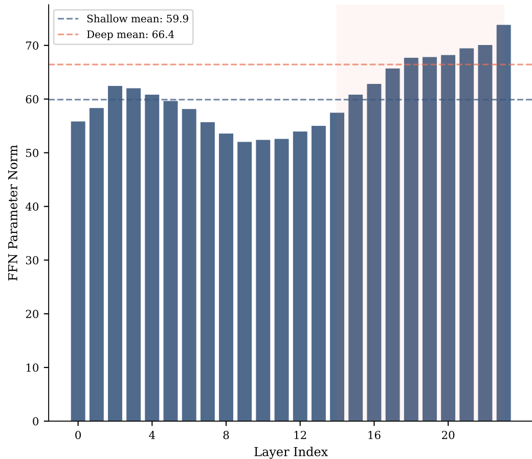
(a) FFN Parameter Norm (Deep/Shallow = 1.11 \times )
