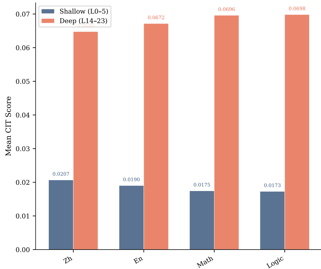
(b) CIT Functional Importance (Deep/Shallow = 3.6 \times )
