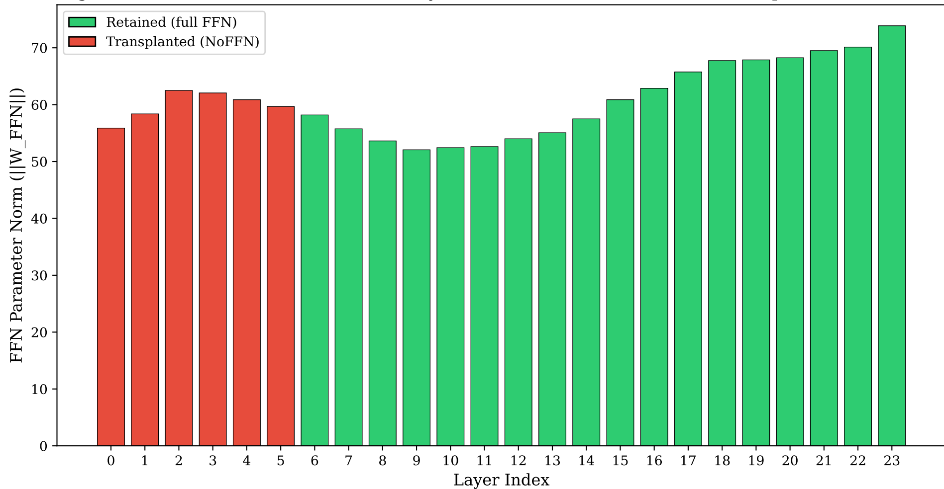
Figure 8: FFN Parameter Norm Across Layers — Green = Retained, Red = Transplanted (Profile P1)
