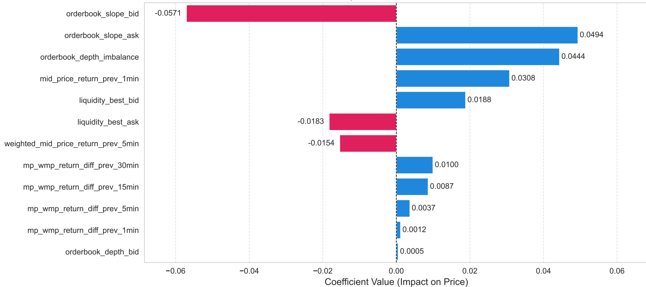
Top Lasso Coefficients
