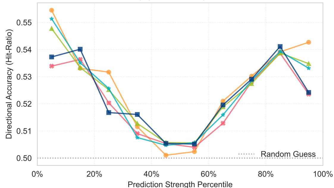
A: Directional Accuracy (10% Q-Bins)
