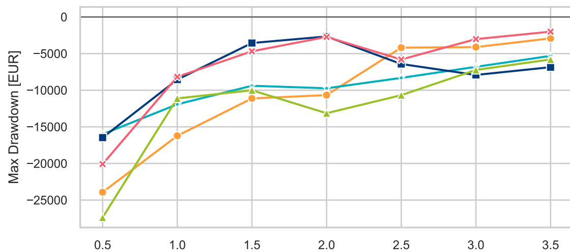
G: Maximum Drawdown
