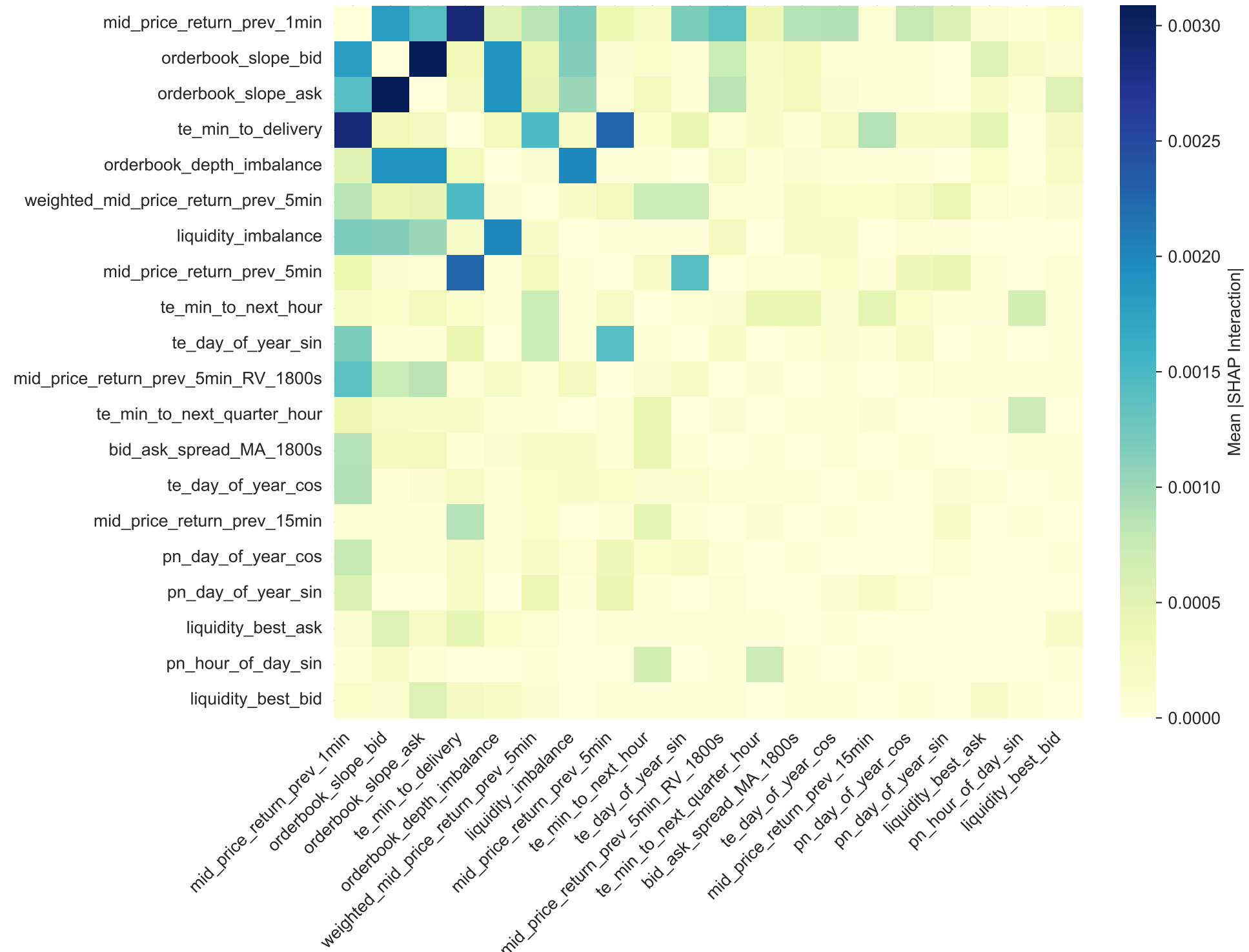
Interactions: CatBoost
