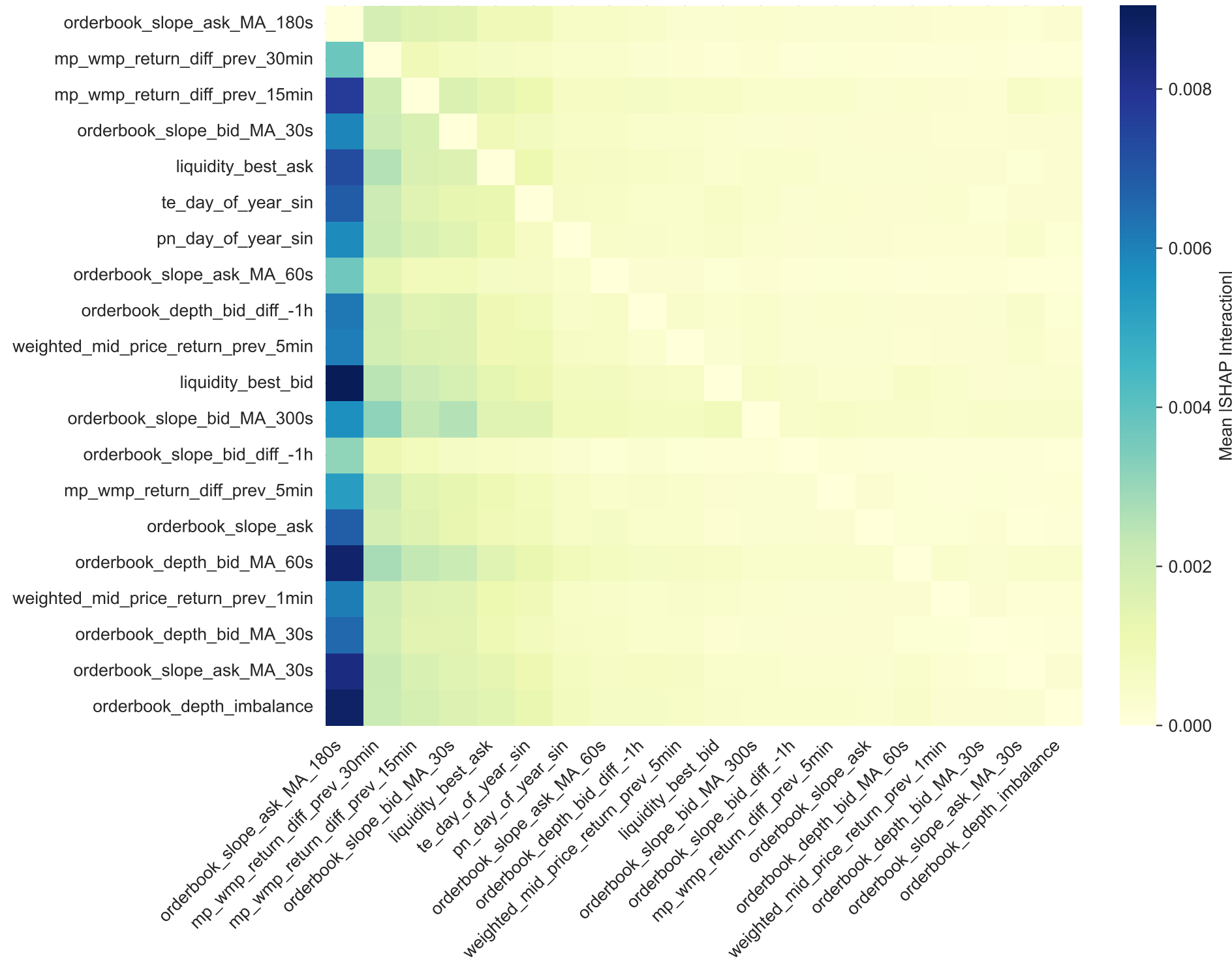
Interactions: RandomForest
