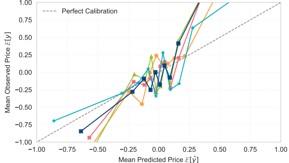
B: Reliability Diagram (10% Q-Bins)
