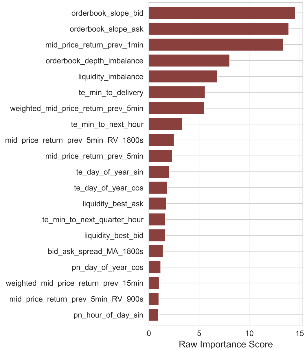
CatBoost (PredictionValuesChange / Raw)
