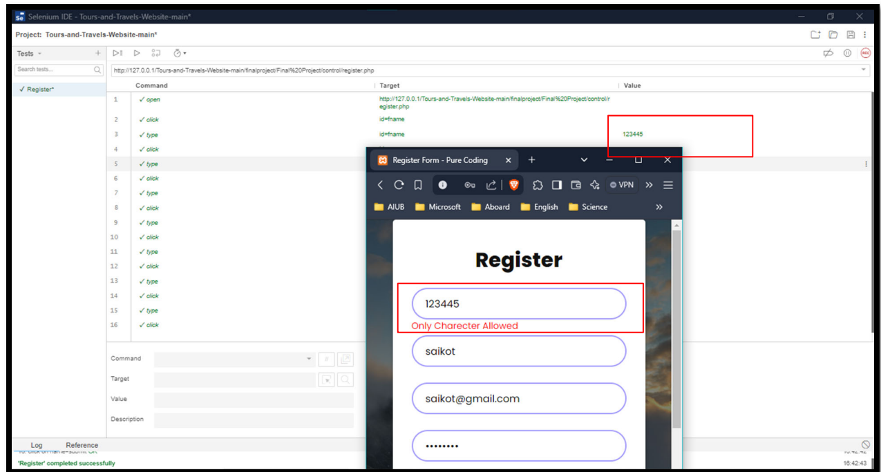
Fig8: Testing with invalid Input (Wrong name)
