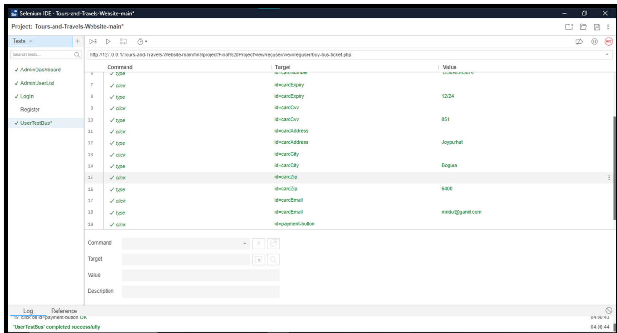
Fig19: Testing the feature for buying a ticket (with all valid field) by a user of the system
