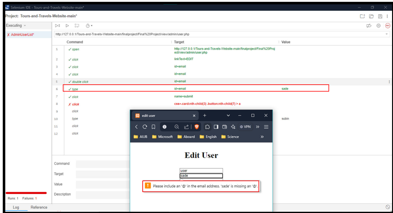
Fig18: Testing the feature “User List” for Admin Module (With Invalid Email)
