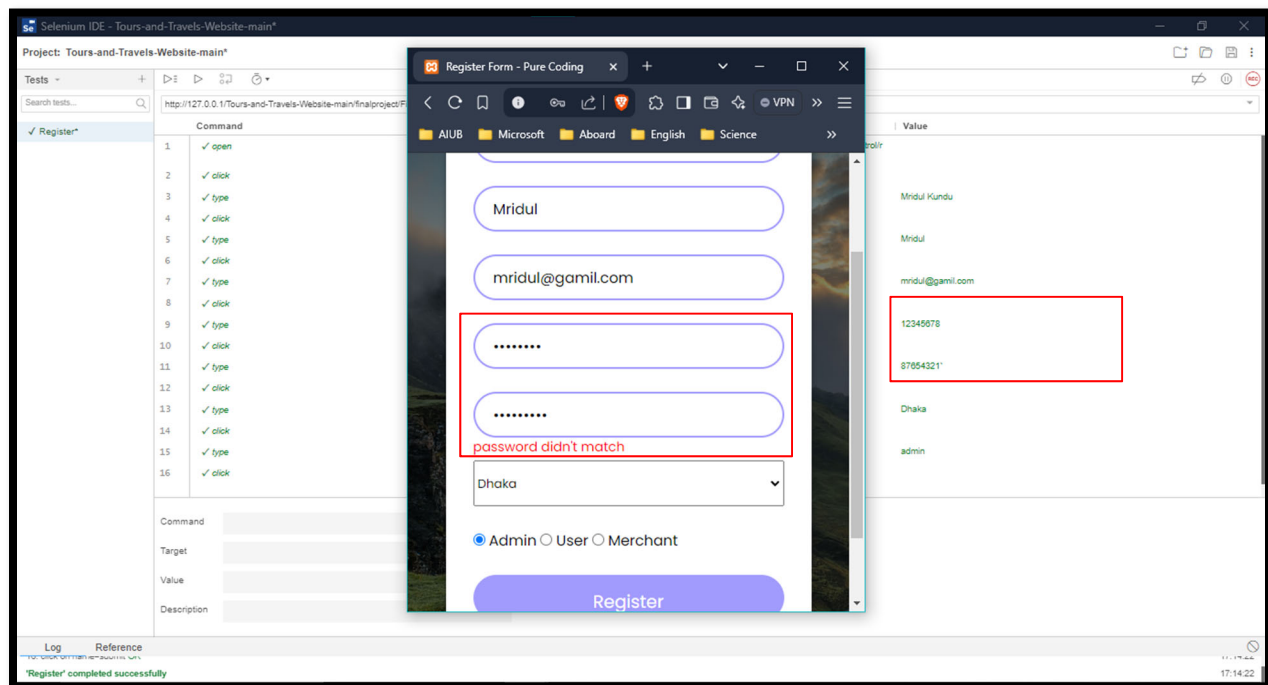
Fig11: Testing with invalid Input (Wrong confirm password)
