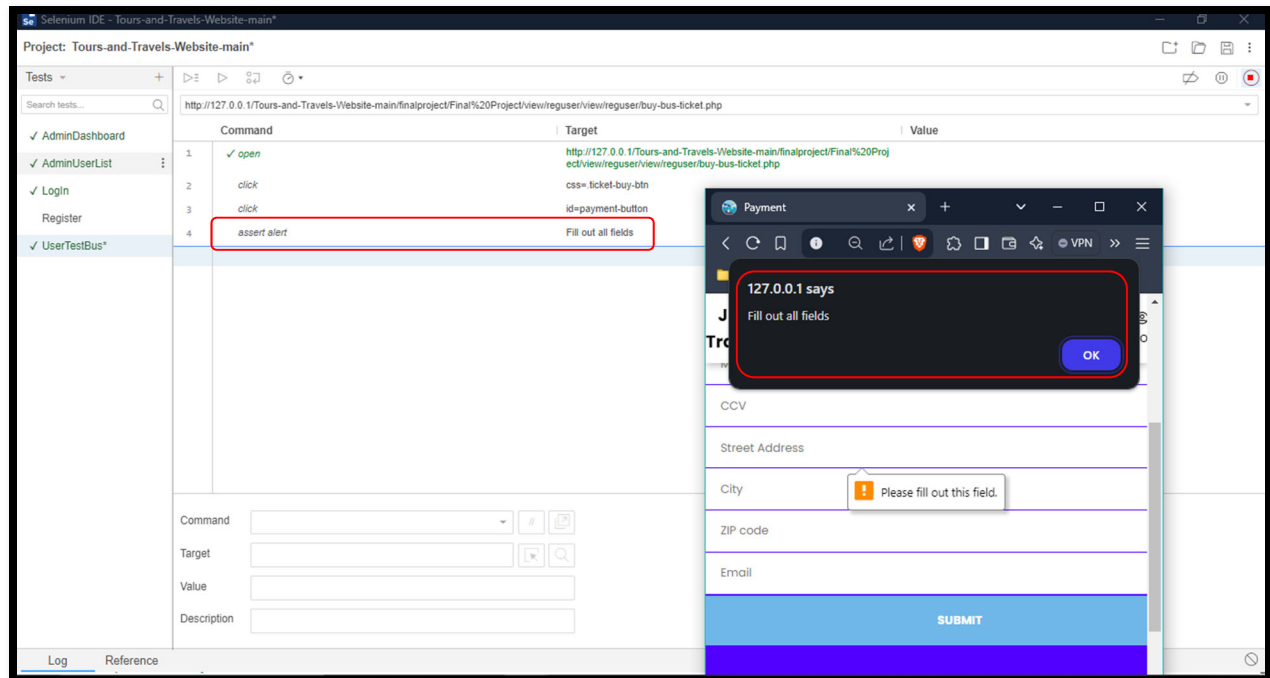
Fig20: Testing the feature for buying a ticket (with all empty fields) by a user of the system
