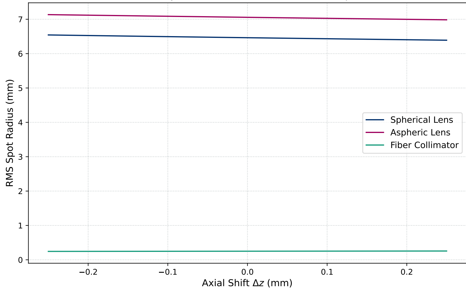
Tolerance Analysis: Effect of Axial Shift on RMS Spot Radius
