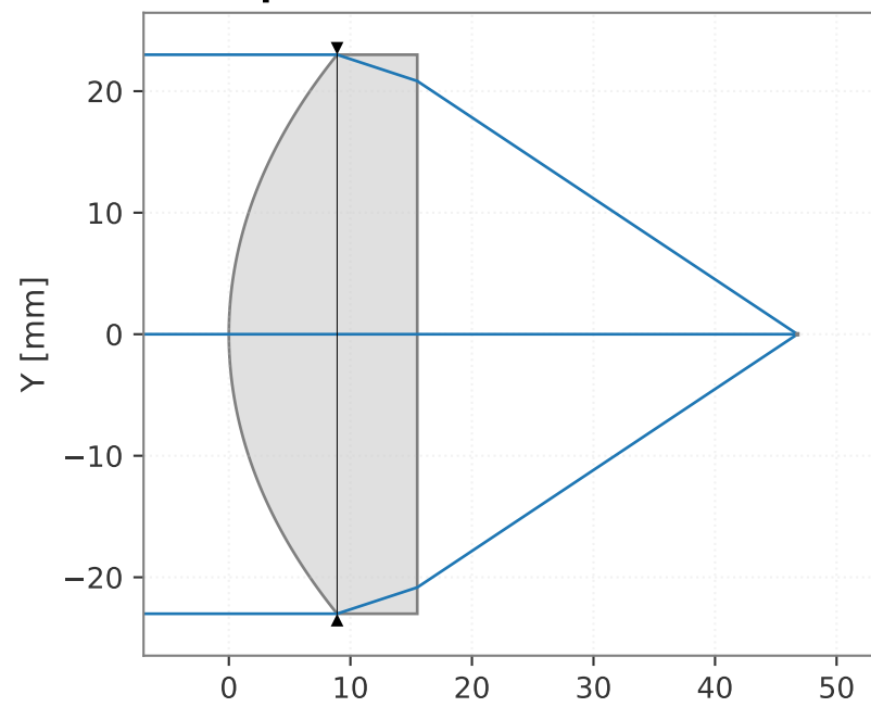
(b) Aspheric Lens (Thorlabs AL5040H-B)
