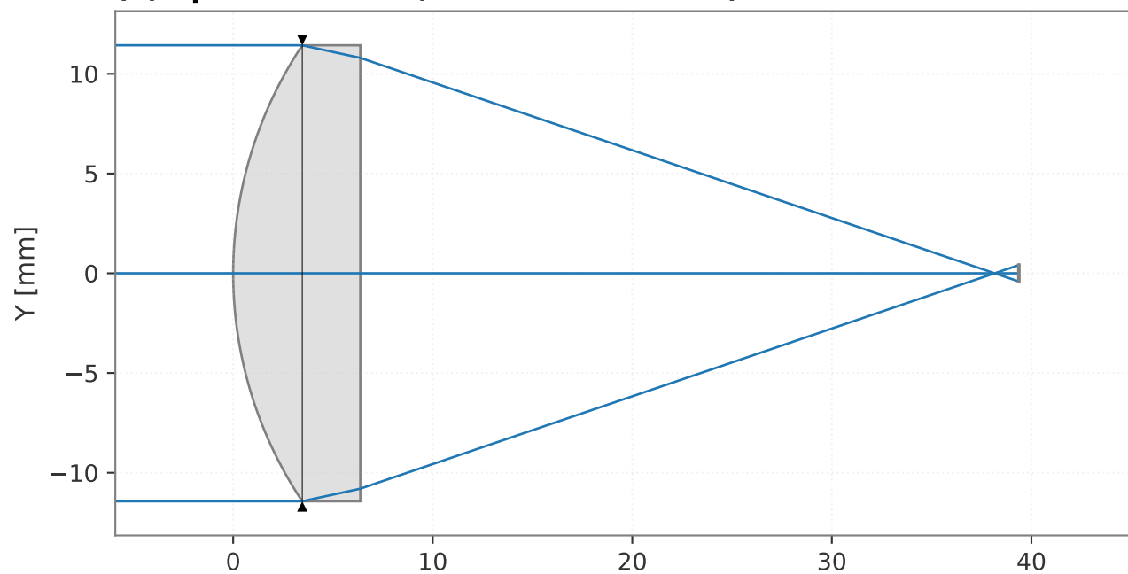
(b) Aspheric Lens (Thorlabs AL5040H-B)
