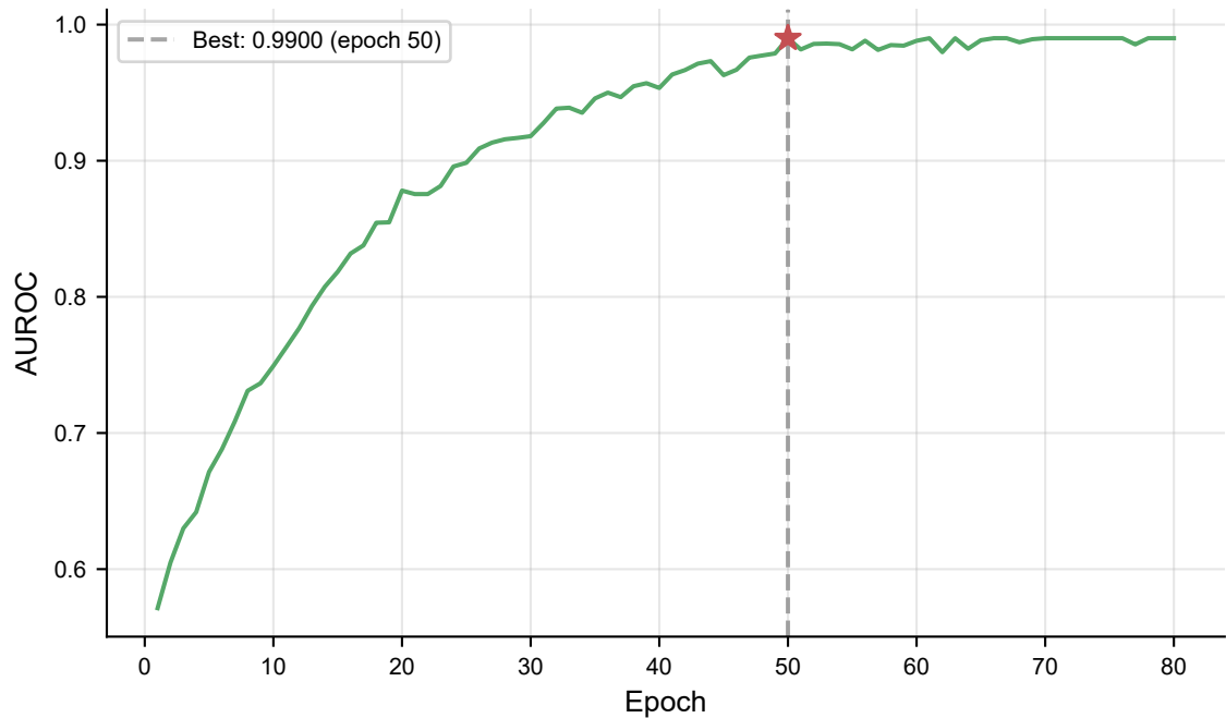
(b) Validation AUROC
