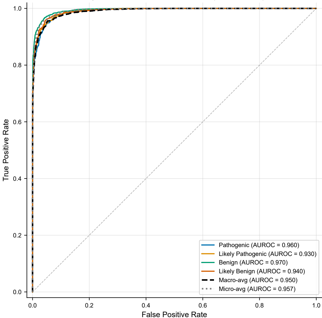
Figure 4: Multi-Class ROC Curves (One-vs-Rest)
